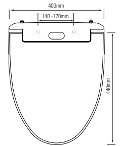
RA-HS Heated Seat
